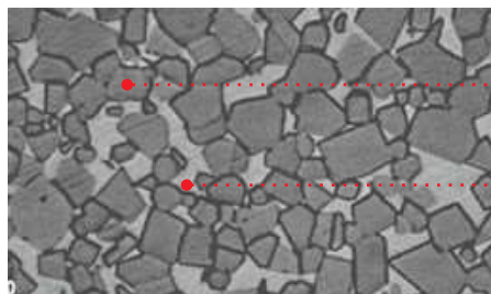
Cemented Carbide(Sintered)
